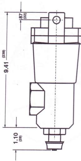
1" AIR DRYER Part No. 020-048-008
