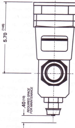
1/2" AIR DRYER Part No. 020-047-007
